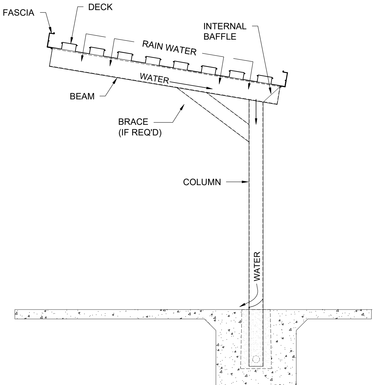
SLOPED CANTILEVERED BENT
