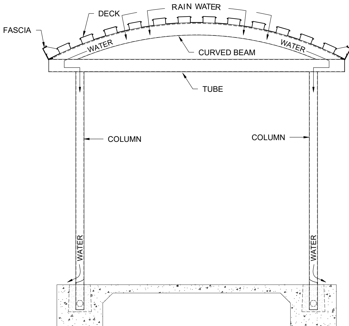
BARREL VAULT U-BENT
