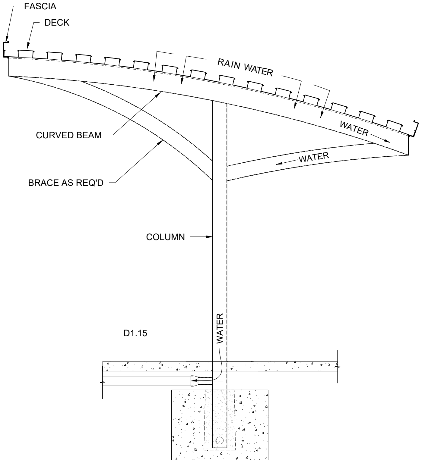
SLOPED BARREL VAULT T-BENT
