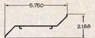
4" Z BLADE
