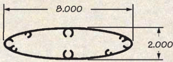
8" ELLIPTICAL BLADE
