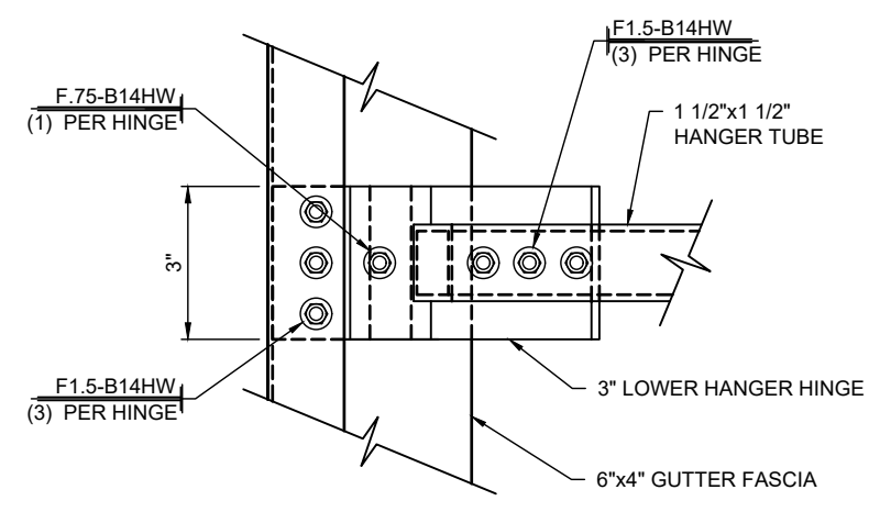
3 CANOPY SECTION 4.03 SCALE: 3"=1'-0" CANOPY: C REF.: NONE
