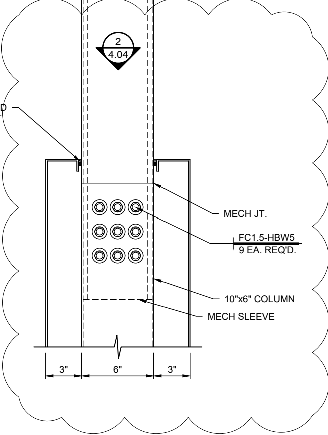
2 4.00 CANOPY BAY BREAK DETAIL SCALE: 1 1/2"=1'-0" CANOPY:B REF.: 1/A6.7 (SIM)
