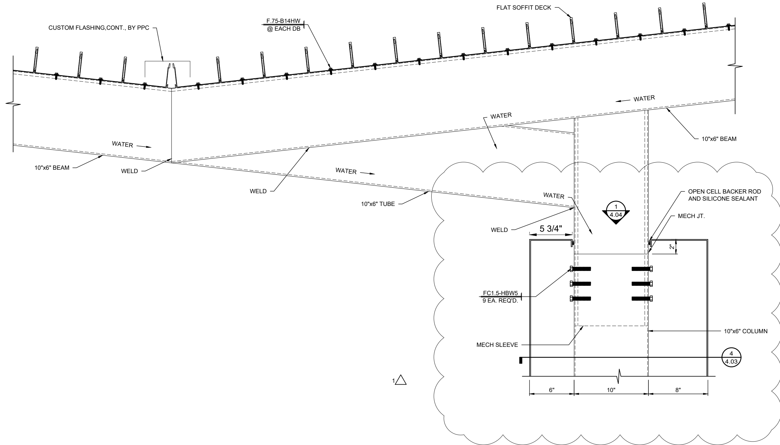
1 4.02 CANOPY MECH JT DETAIL SCALE: 1 1/2"=1'-0" CANOPY: A REF.: 5 & 6/A6.7
