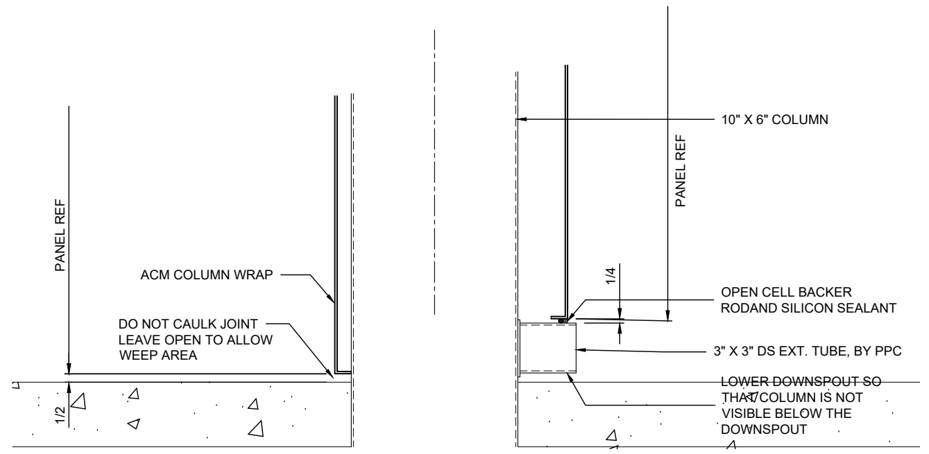
3 COLUMN DETAIL @ DOWNSPOUT 4.04 SCALE: 1 1/2"=1'-0" CANOPY: A REF.: NONE
