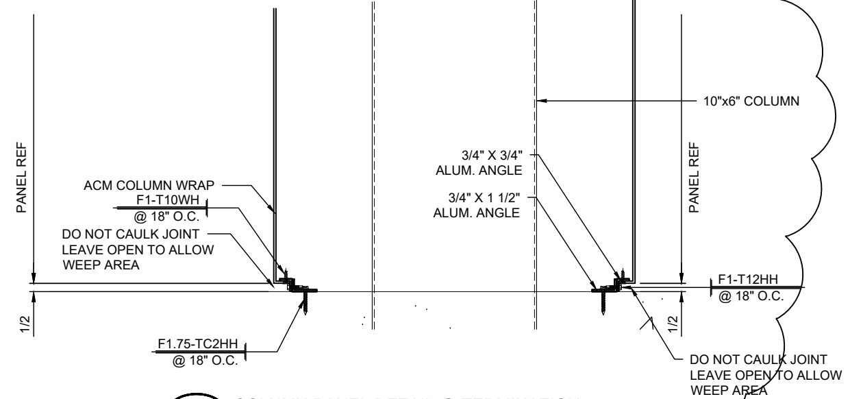
4 COLUMN PANEL DETAIL @ TERMINATION 4.04 SCALE: 1 1/2"=1'-0" CANOPY: B REF.: NONE
