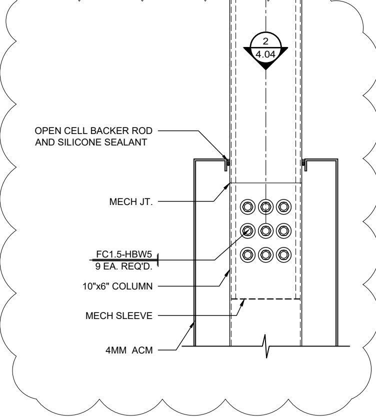
3 4.00 CANOPY END DETAIL SCALE: 1 1/2"=1'-0" CANOPY:B REF.: NONE
