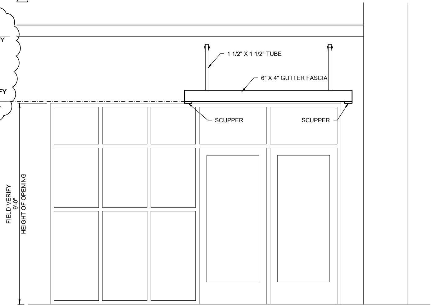
3 ELEVATION SCALE: 3/8"=1'-0" CANOPY:C REF.: 2/A3.0
