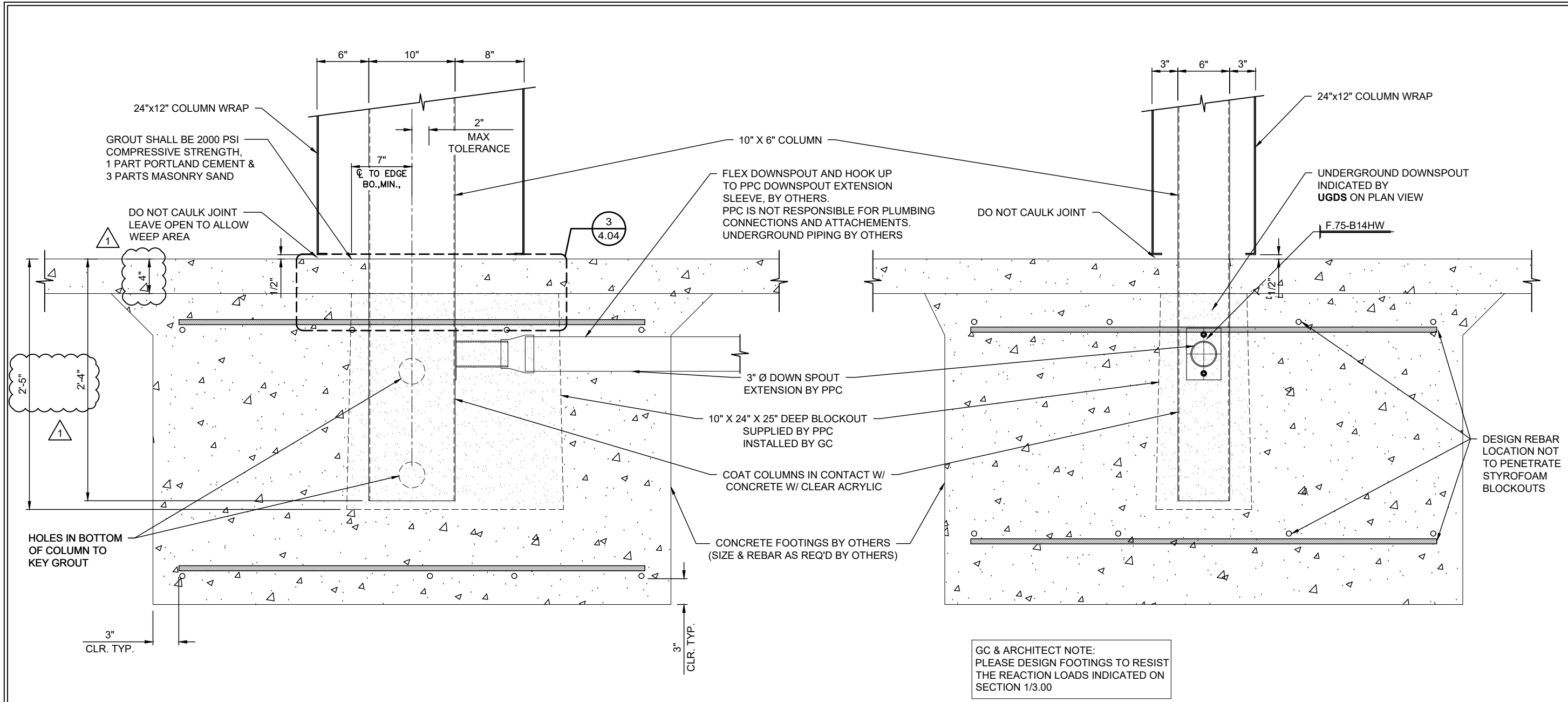
1 BLOCKOUT DETAIL 5.00 SCALE: 1"=1'-0" CANOPY: A REF.: 4/A6.7
