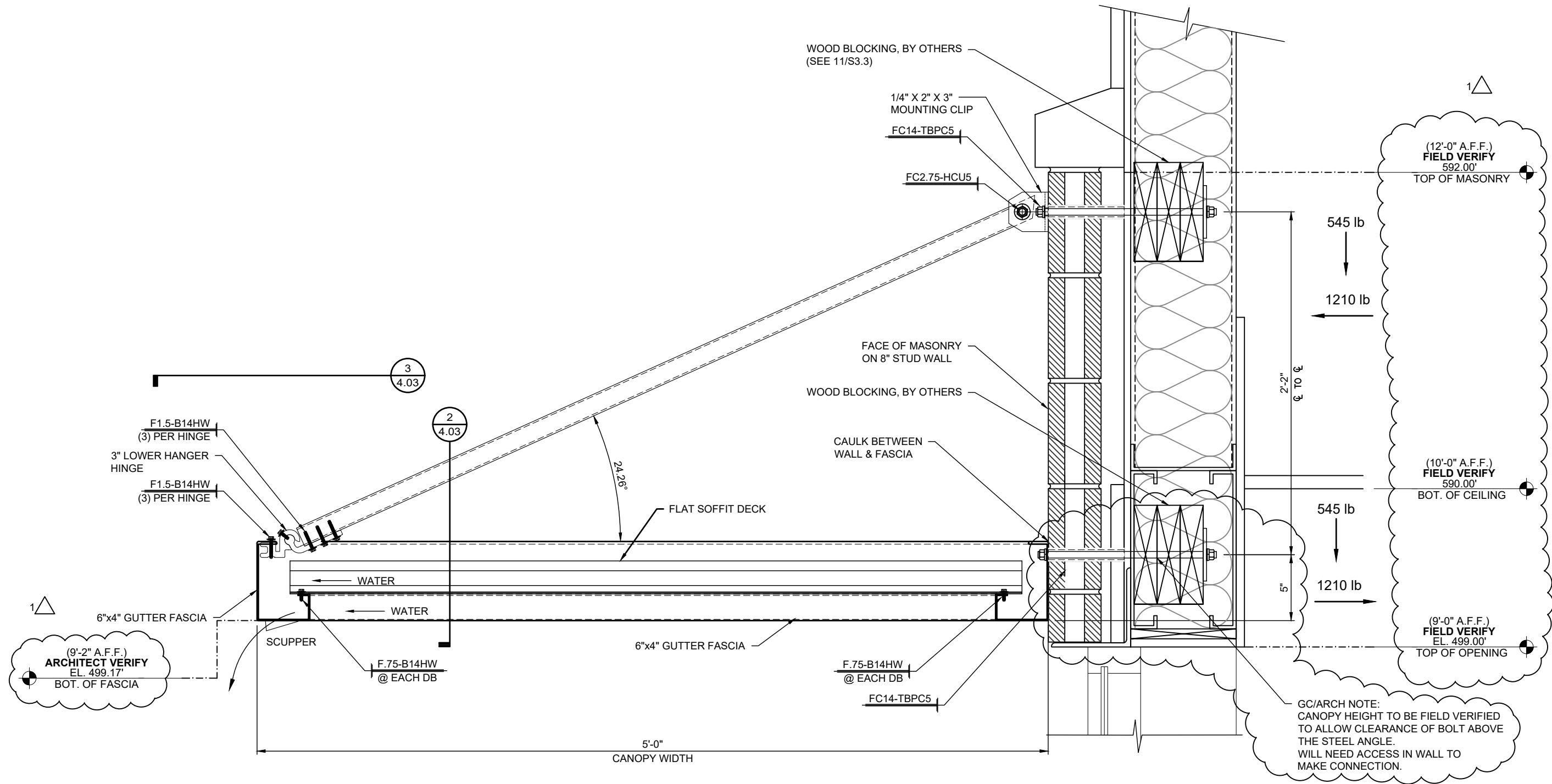
1 3.01 CANOPY SECTION SCALE: 1 1/2"=1'-0" CANOPY: C REF.: 2 & A/A6.1, 8/A6.7 & 11/S3.3
