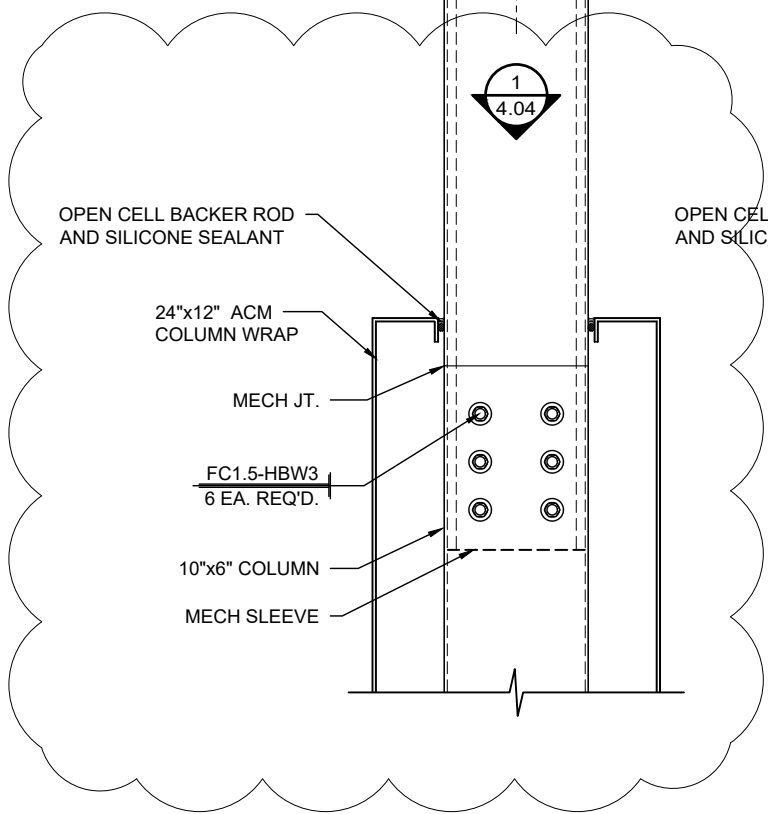
1 4.00 CANOPY END DETAIL SCALE: 1 1/2"=1'-0" CANOPY:A REF.: NONE
