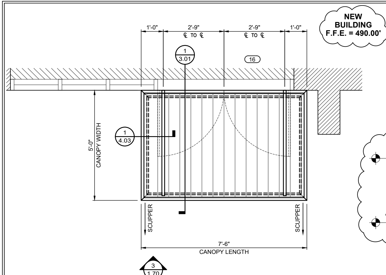
1 DECK PLAN SCALE: 3/8"=1'-0" CANOPY:C REF.: 1/A1.0 & A9.0
