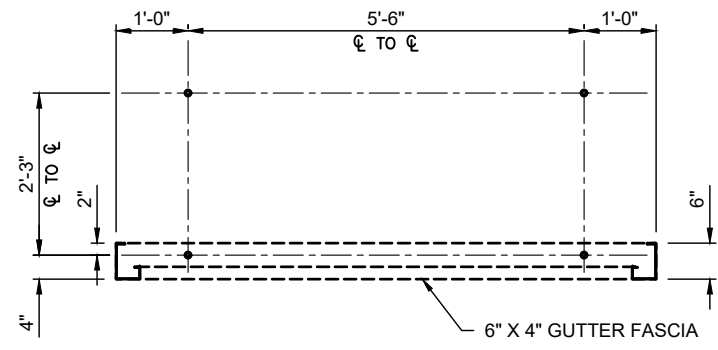
2 BOLT SETTING PLAN SCALE: 3/8"=1'-0" CANOPY:C REF.: C/A3.0
